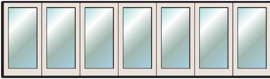
30" Doors 17' 6" wide (R/O 214")
